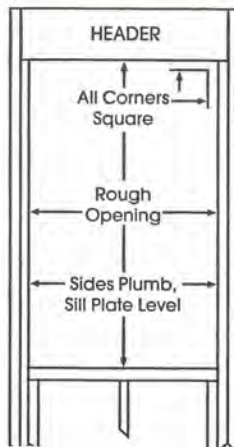
FIG. 2 INTERIOR VIEW
