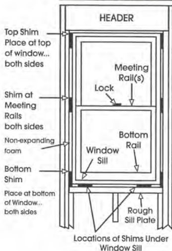
FIG. 2 INTERIOR VIEW
